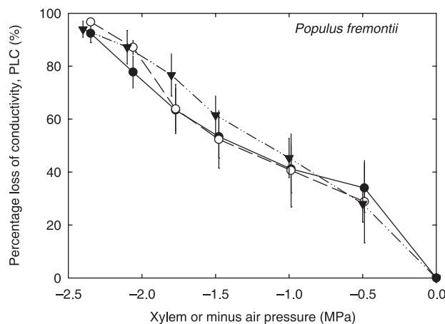
Fig. 5 Vulnerability curves for diffuse-porous Populus fremontii using the spinning (open circles) and gravity (closed circles) methods on the same stem segments, and the air-injection method (triangles) on separate segments. Conductivity is plotted as per cent loss from initial value (PLC) to facilitate comparison with the air-injection method used on separate stems. None of the means were different. Mean \pm SE for six stems.
