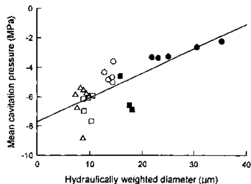
Fig. 3. Linear regression of mean cavitation pressure vs hydraulically weighted tracheid diameter. Pinus edulis branches ( \circ ) and roots ( \bullet ), J. osteosperma adult branches ( \square ), roots ( \blacksquare ) and juvenile branches ( \triangle ); r^2 = 0.58 .
