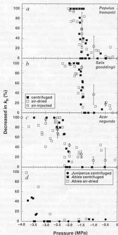
FIG. 1 Decrease in hydraulic conductivity ( k_h ) in xylem against xylem pressure ( \Psi_{px} ) generated by centrifuging (filled symbols) and air-drying (open symbols) stems of a, Populus fremontii , b, Salix gooddingii , c, Acer negundo and d, Abies lasiocarpa . Centrifuge data only are shown for Juniperus monosperma (d). Decrease of k_h from air injection of xylem (a-c, open circles) is shown against the negative of the injection pressure for comparison. All species were from Pima County, Arizona, except A. lasiocarpa from the Wasatch Mountains of Utah. METHODS. In centrifuge experiments, stems were re-cut underwater to a length (26–40 cm) several times longer than all or most of the conduits in each species (W.T.P. and J.S.S., unpublished observations). The bent ends that centre the water column in z-tubes 20 were unnecessary because of capillarity at inter-conduit pits. Initial k_h of each segment was measured using a method described previously 30 . The stem was centred on the rotor of a centrifuge (Sorvall, GLC-1) and spun to generate a pressure ( P ): P = 0.5 \sigma \omega^2 r^2 , where \sigma is the density of water, \omega is the angular velocity ( \text{rad s}^{-1} ) and r is half the total stem length (cm) 19,20 . Angular velocity was determined using the centrifuge tachometer. After 4 min (2 min for A. lasiocarpa ) centrifugation, stems were left in damp paper towels for 20–60 min to allow air to diffuse into vapour-filled conduits. Final k_h was measured after removing 2–5 cm from each end under water to eliminate blockage by drained, severed conduits. Cavitation was expressed as the percentage decrease of final k_h from its initial value. The centrifuge was too slow to completely cavitate Abies or Juniperus . In air-drying experiments, decrease in k_h was calculated from native and flushed k_h 30 , and xylem pressure was measured with the pressure chamber. Air-injection experiments were performed as described previously 25 .
