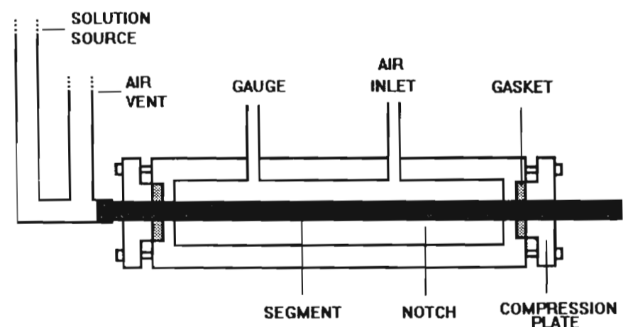
Figure 1. Apparatus for measuring vulnerability curves on single hydrated stems using air pressure. The stem (SEGMENT) was sealed in a double-ended steel bomb with both ends protruding. Rubber gaskets were fitted around the stem and held in recessed wells. An air-tight seal was made by screwing on compression plates and squeezing the gasket around the stem. Although we used a variety of bomb designs, the one shown was the latest and the most efficient. Air pressure in the bomb was controlled with a regulator and measured with a test gauge via a separate port. The separate measurement port avoided errors resulting from the pressure drop along the inlet flow route. An intravenous bag was used as a solution source fitted to the stem with clear tubing (SOLUTION SOURCE); elevation of the bag forced solution through the segment under gravity during conductance measurements. Effluent was collected using pre-weighed vials containing cotton wool. An open-ended tube allowed escape of air during pressurization (AIR VENT).
